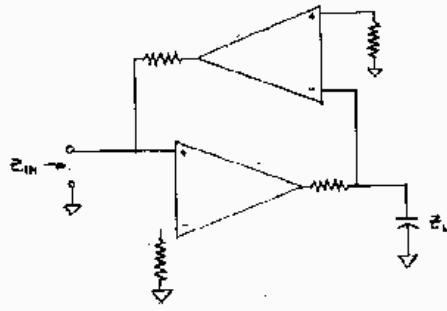
FIG 3 - SIMPLE GYRATOR
